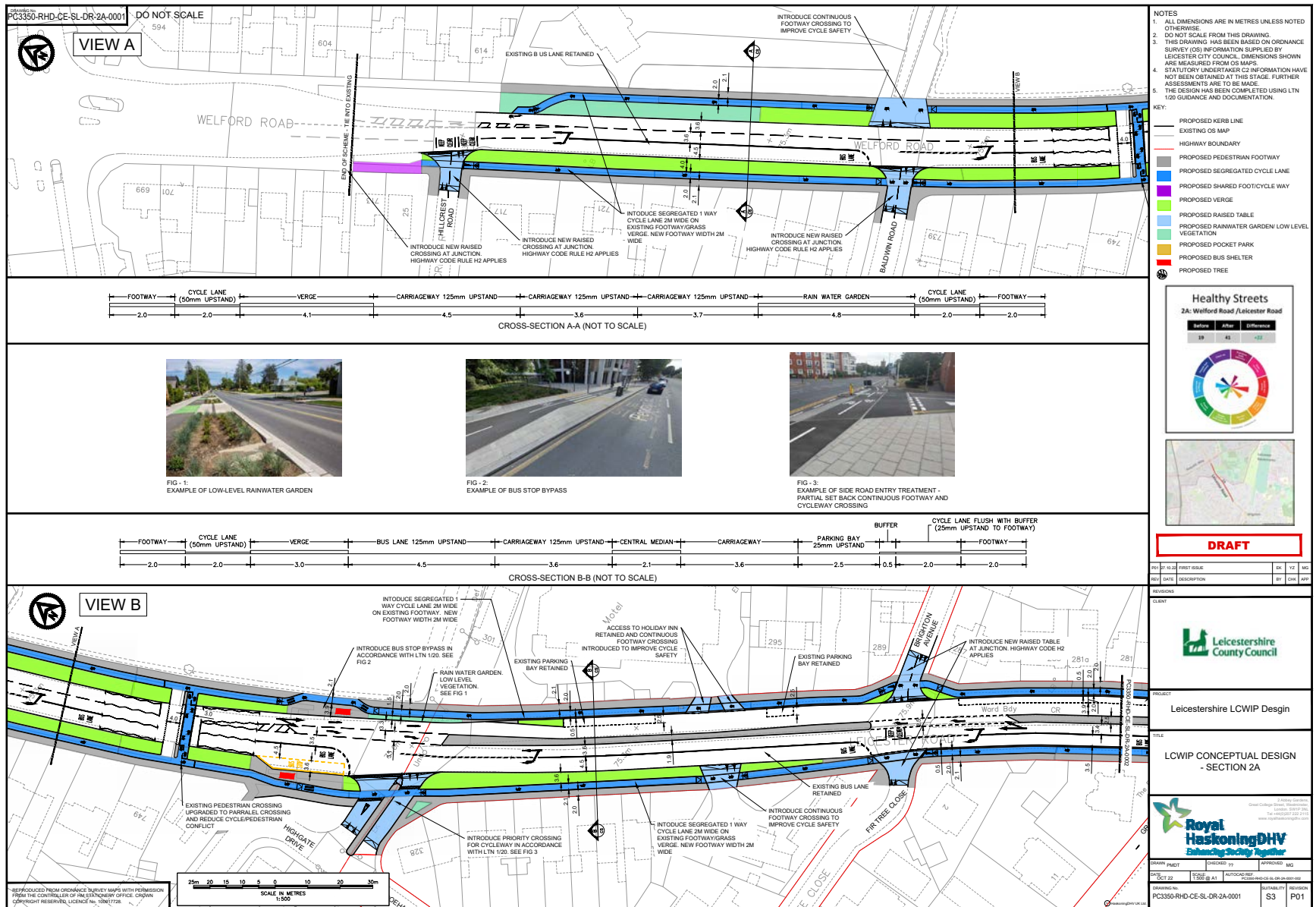
Figure 7.13 – Concept design for route section 2A (Leicester Road / Bull Head Street)
