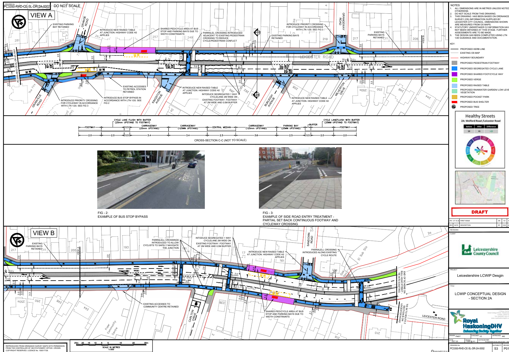
Figure 7.9 – Concept design for route section 2A (Leicester Road / Bull Head Street)
